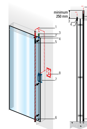
GLASS DOOR WITH ELECTRIC LOCK (SOLUTION ON WALL)
