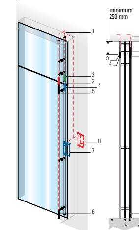
GLASS DOOR WITH ELECTRIC LOCK (TOP WINDOW SOLUTION)
